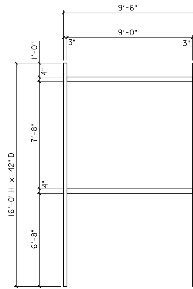
(STANDARD BAY) 108" RACK
