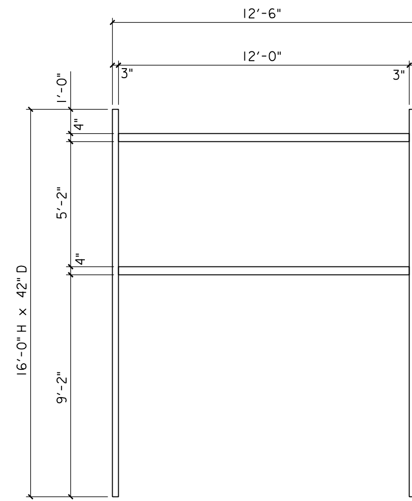
(BRIDGE BAY) 144" RACK
